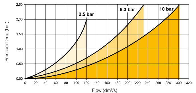
(3/4) 0.01µm Coalescing Filter Saturated
