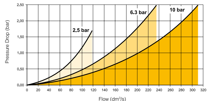
(1") 0.01µm Coalescing Filter Saturated
