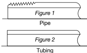
Figure 2 With no threading necessary, tubing does not require extra wall thickness
